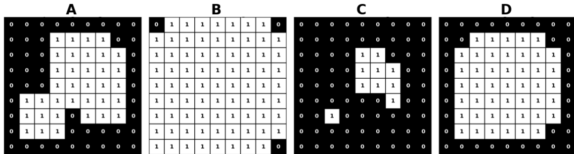
Figure 3: Morphological operation results on the input binary image.
