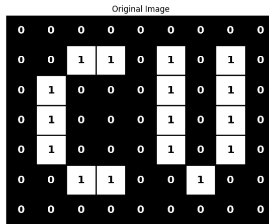
Figure 4: A binary image for connected component analysis.
