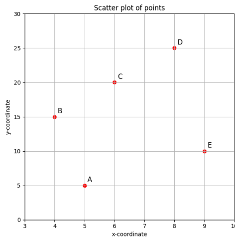
Figure 6: Scatter plot of points
