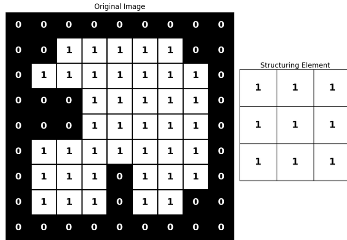
Figure 2: Input binary image and structuring element.
